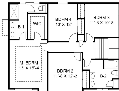
SECOND FLOOR 1041 S.F.
