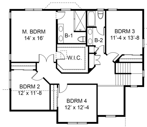
SECOND FLOOR 1215 S.F.
