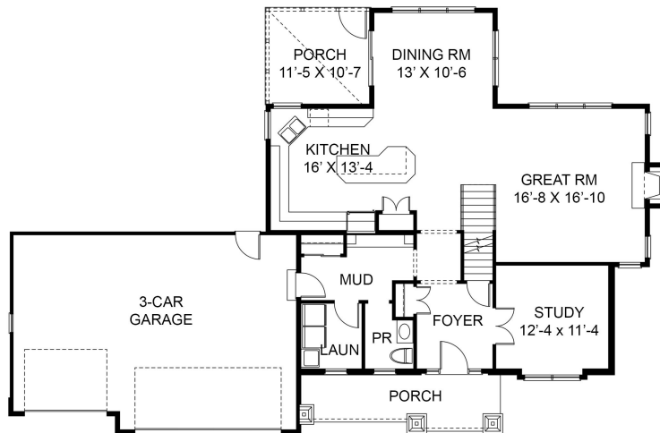
FIRST FLOOR 1294 S.F.
