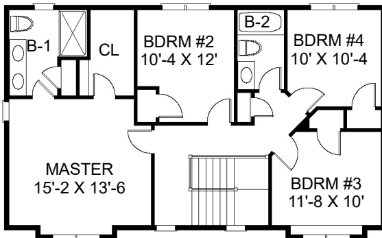
SECOND FLOOR 922 S.F.
