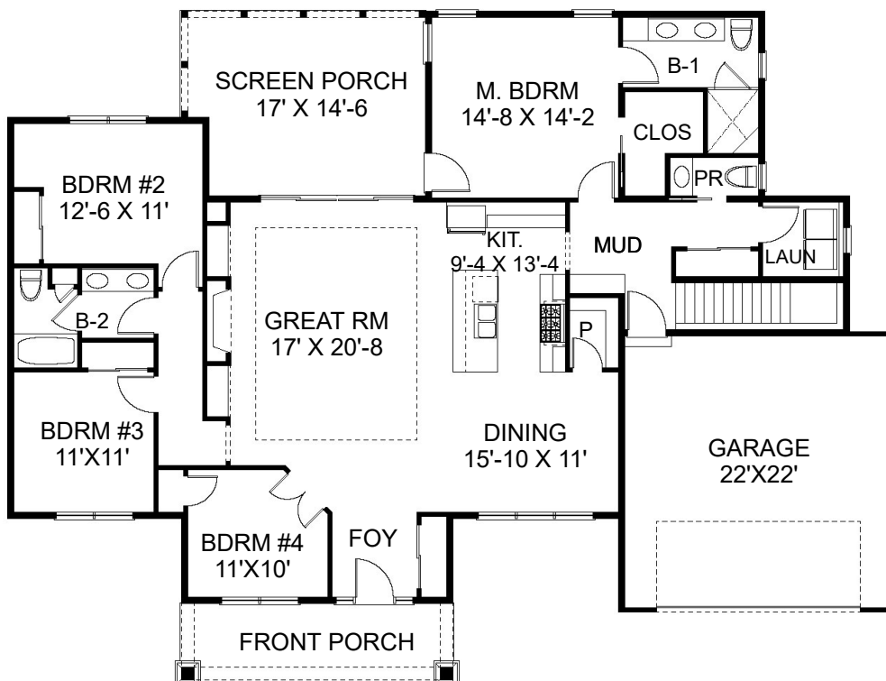
FLOOR PLAN AREA: 2050 S.F.
