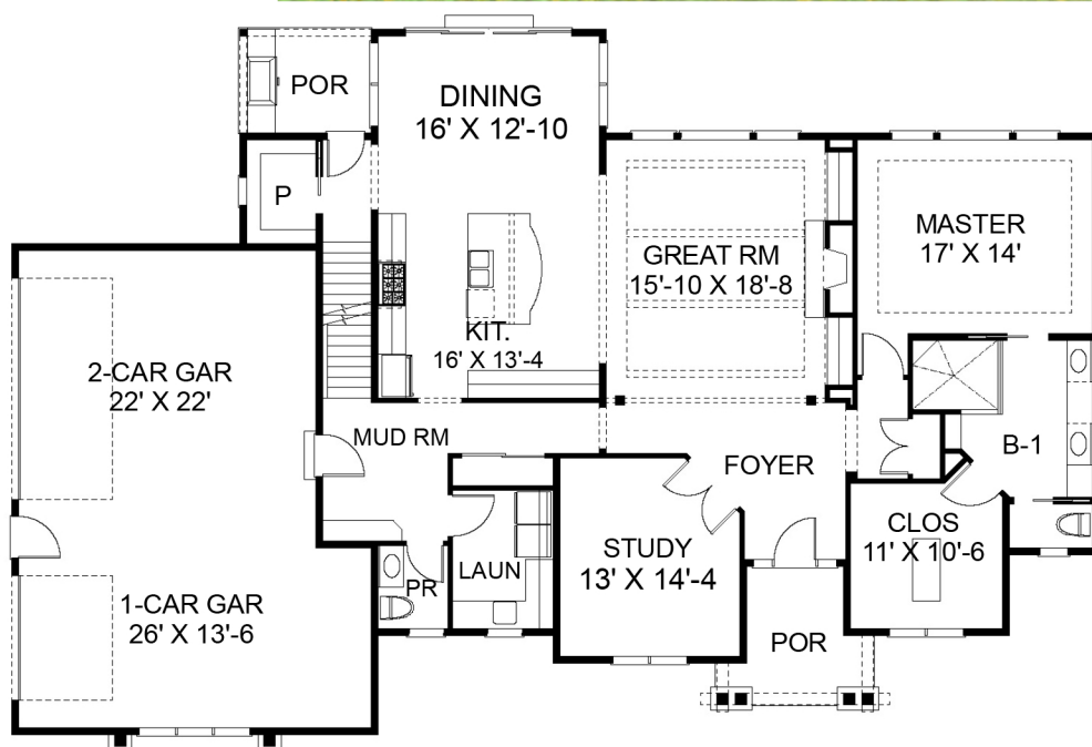
FIRST FLOOR 2163 S.F.
