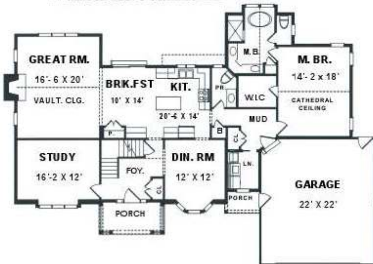
FIRST FLOOR AREA: 1738 SQ. FT.
